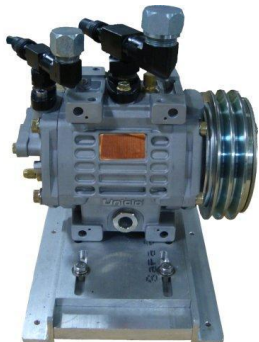
BELT DRIVEN COMPRESSOR off main engine approx dimensions: 11"w x 19"l x 12"h (includes adjustable base for belt tightening)
